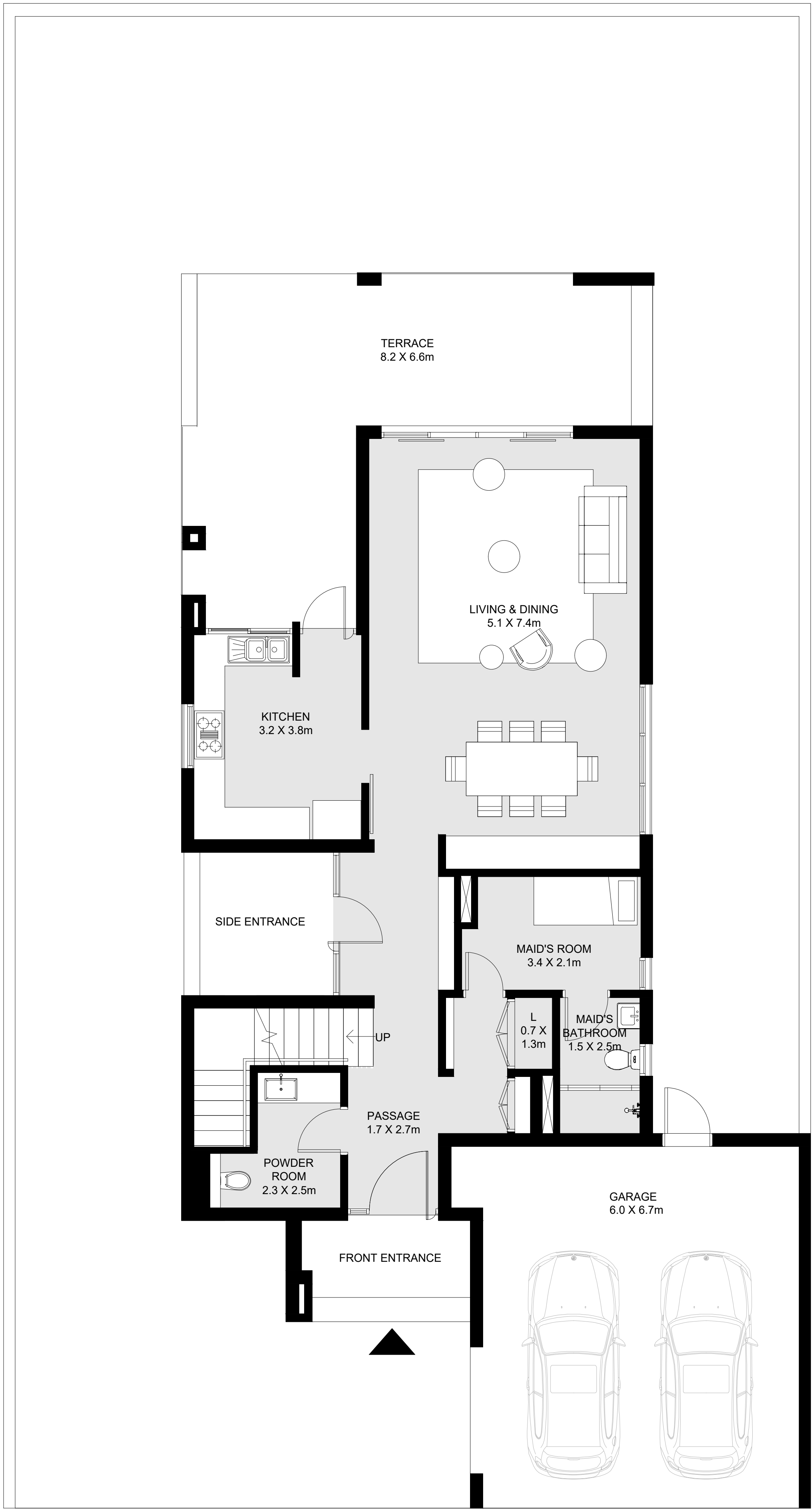
GROUND FLOOR
