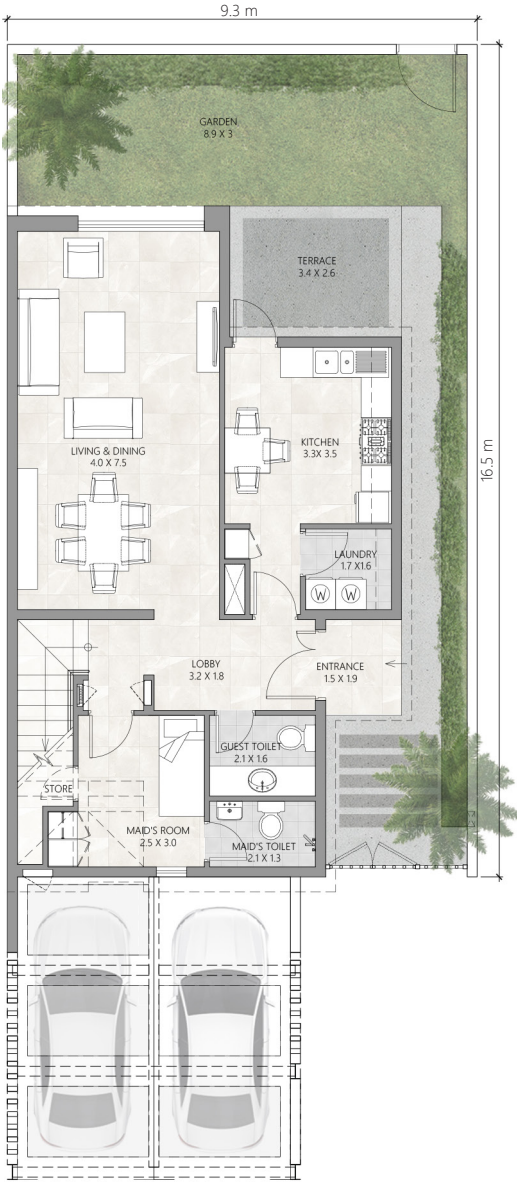
GROUND LEVEL PLAN
